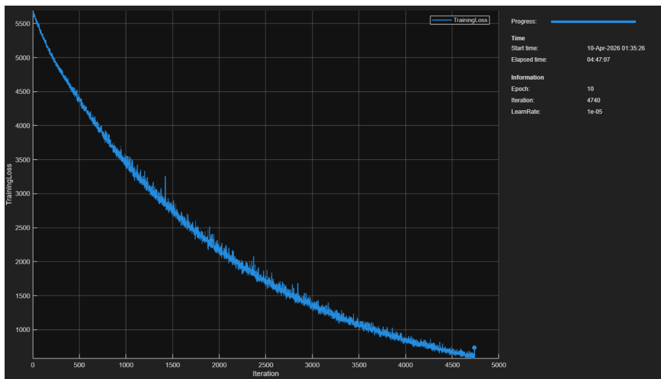
Figure 5.3: YOLOv4 Training Progress - Loss Convergence over Epochs
